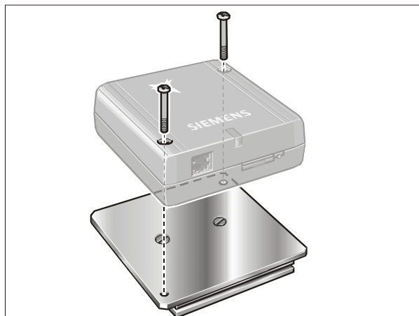
Figure 12: Attaching TC35i Terminal to a top-hat rail
