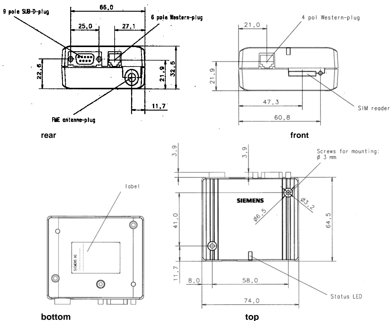
Figure 10: Design drawing
