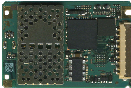
Figure 2: TC35i GSM engine
